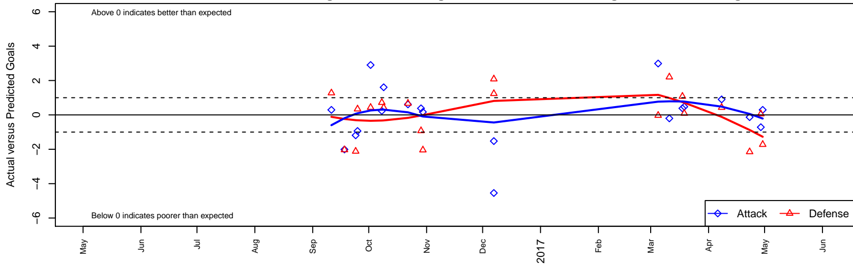
BSC HR Black B04 Dots are actual minus expected GF (blue circles) and GA (red triangles). Blue line is smoothed change in attack strength. Red is smoothed change in defense strength.
